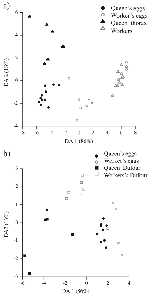
Fig. 2 Discriminant analysis of a cuticular HC profiles of queens' thoraces ( filled triangle ), entire workers ( empty triangle ), queen-laid eggs ( filled circle ), and worker-laid eggs ( empty circle ); b Dufour HC and alkaloids profiles of queens' glands ( filled square ), workers' glands ( empty square ), queen-laid eggs ( filled circle ), and worker-laid eggs ( empty circle ). The percentage of variance explained by the first two discriminants is given for each axis
